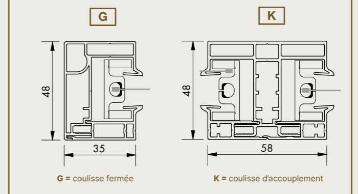
Coulisses
