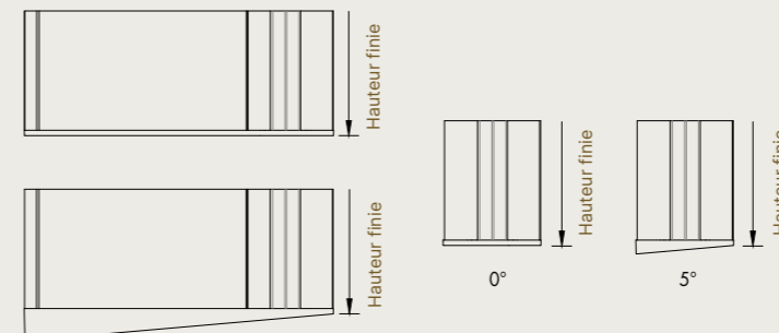
Plaque de base
